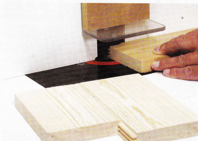
10 The Wealden finger joint cutter, assembled to edge-joint 20mm thick boards
