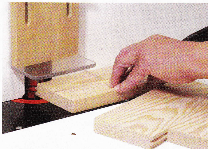
9 Cutting a reverse glue joint. A completed joint can be seen in the foreground
