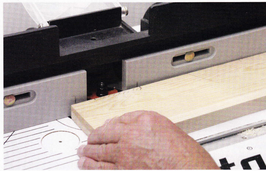
7 Pivoting the board into the cutter. Note pencil marks on fence. The guard is raised here for photographic clarity
