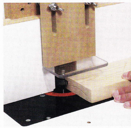
8 Cutting the groove with the cut centred in the board thickness
