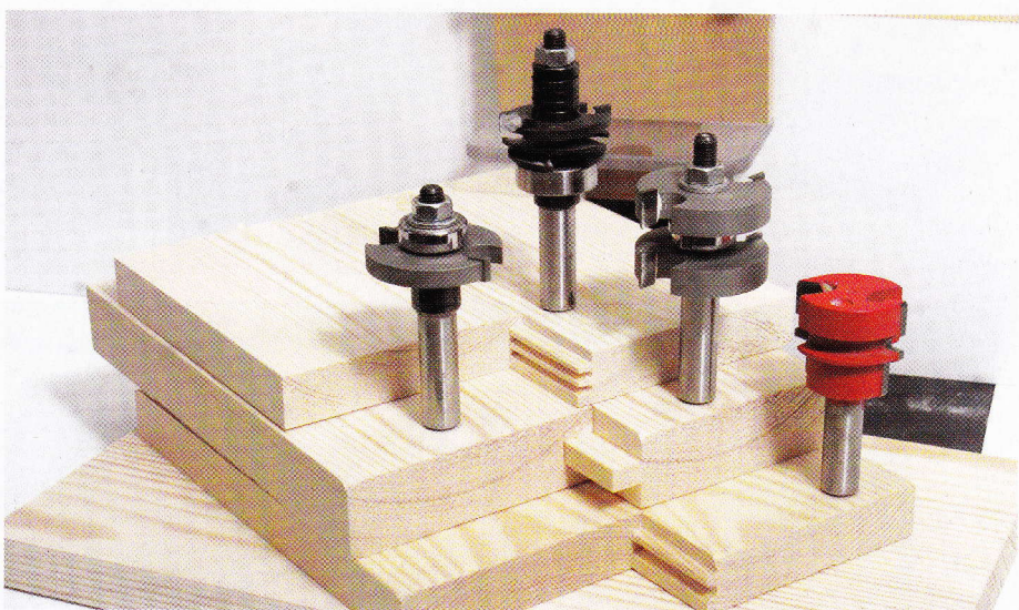
11 Three special joint cutters and joints made with them
